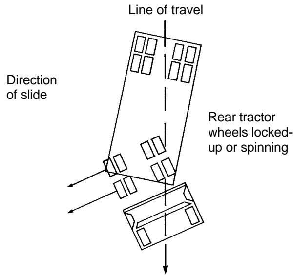
Figure 6-2 Tractor Jackknife
